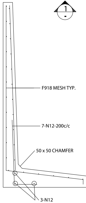
TYPICAL SECTION
